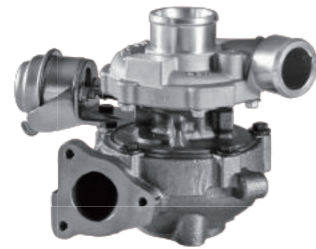
MODEL: GT1544V PART NO. 753420-5005S CAR MODEL: FOR PEUGEOT
